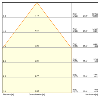
HB P 150W 840 110DEG IP66 PS - REFRACTOR
