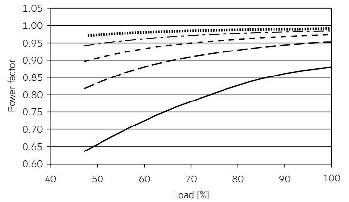
4.6 Power factor vs load (LV)
