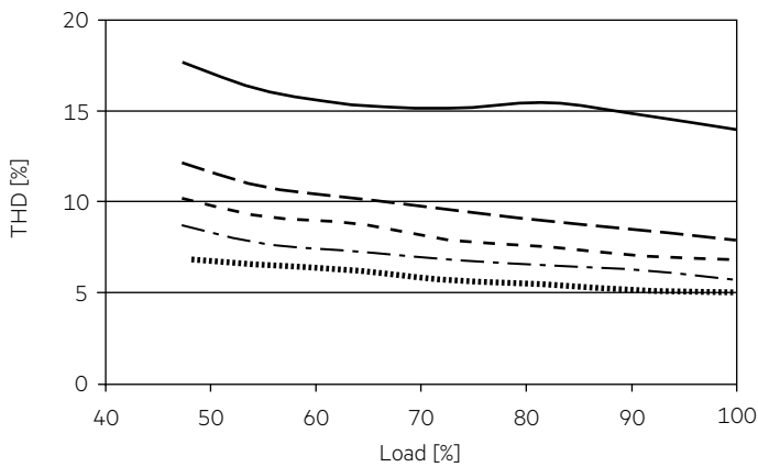
4.7 THD vs load (LV)
