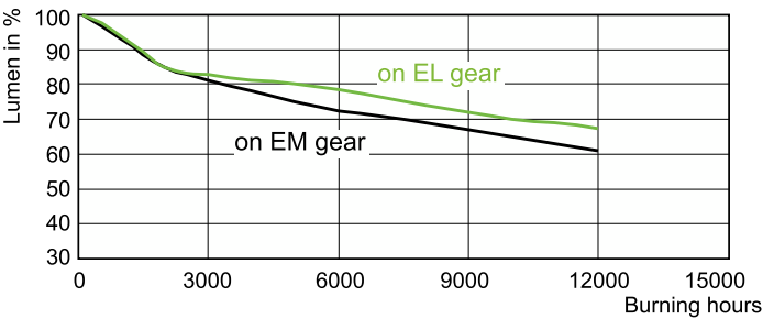
Lumen Maintenance Diagram - MASTER CDM-T 150W/942 G12 1CT
