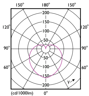
Light Distribution Diagram - CorePro LEDbulb ND 4.9-40W A60 E27 940
